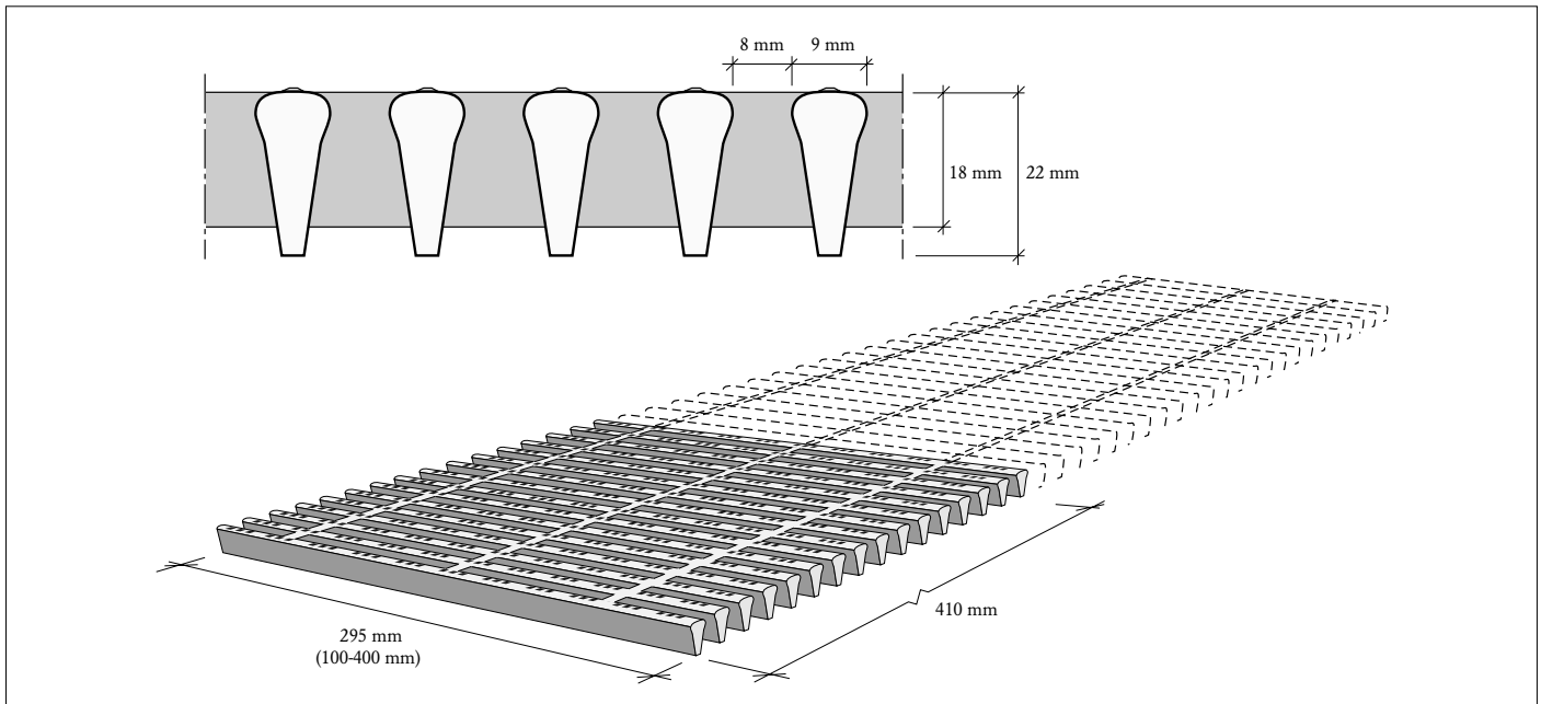
Standard section, designation 024/76
