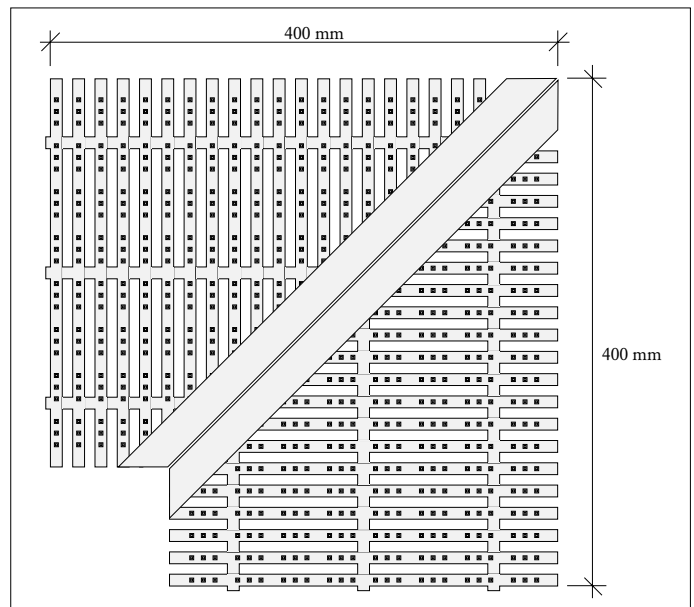
Corner section, designation 024/76/90
